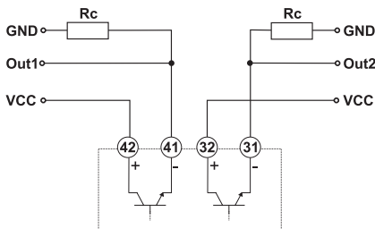
Fig. 25 Static outputs, VCC reference
