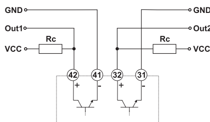
Fig. 24 Static outputs, GND reference
