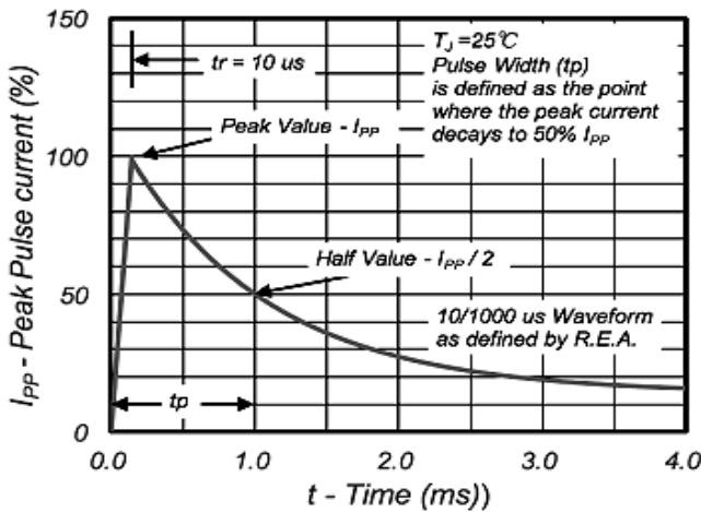
Fig 2: Pulse Waveform
