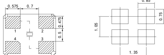
suggested solder pad layout
