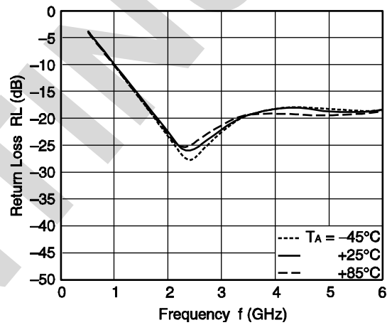
RF1/RF2 RETURN LOSS vs. FREQUENCY
