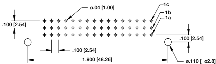
Recommended PCB Layout - Female
