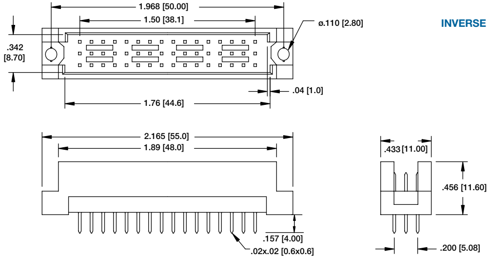
DIN-48FR-S33-A1C1 INVERSE DIN TYPE 1/2 R FEMALE 3 ROW STRAIGHT
