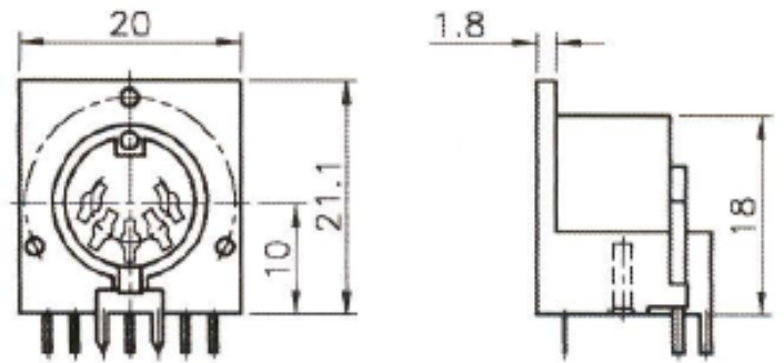
DS-025-3PIN / DS-025
