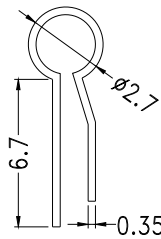
HOLE IN P.C.B \phi 0.8 \sim 1.0
