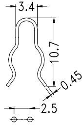
MOUNTING HOLE HOLE IN P.C.B \phi 0.8 \sim \phi 1
