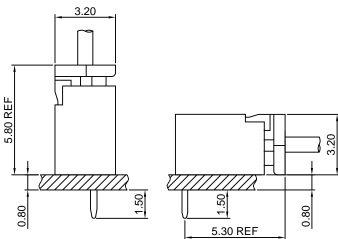
DIP TYPE
