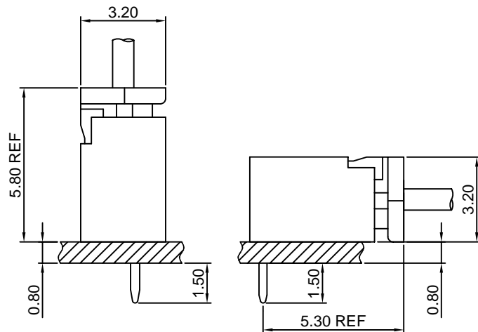
DIP TYPE
