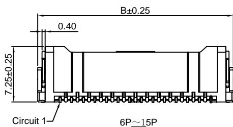
6P~15P Circuit 1
