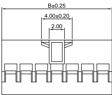
2x3P~2x17P
