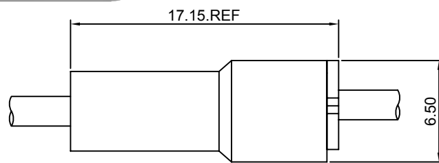
wire to wire
