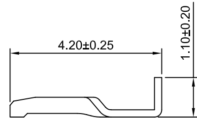
SEC:C-C
