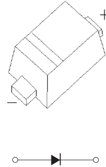
SOD-723
