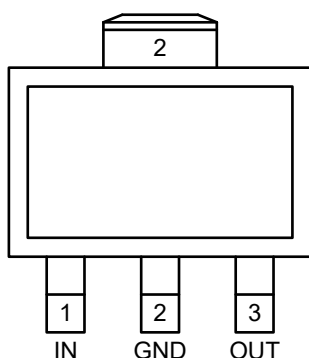
CJ6330AxxG SOT-223
