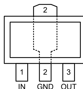
CJ6330AxxPL SOT-89-3L
