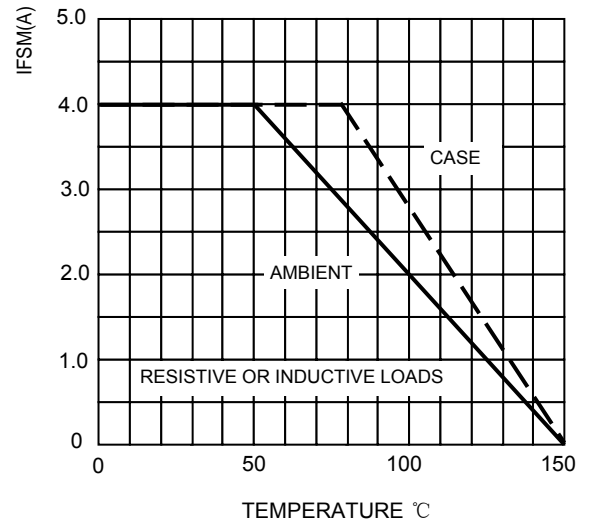
FIG.2-FORWARD DERATING CURRENT
