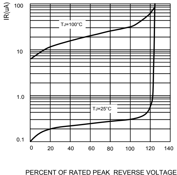
FIG.4-TYPICAL REVERSE CHARACTERISTICS
