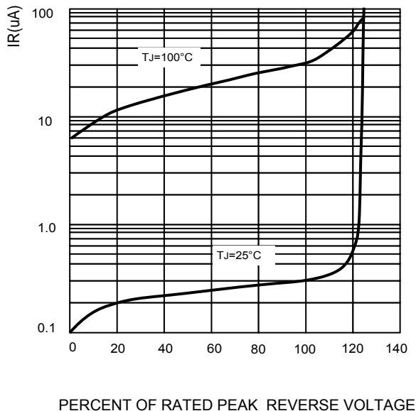
FIG.4-TYPICAL REVERSE CHARACTERISTICS
