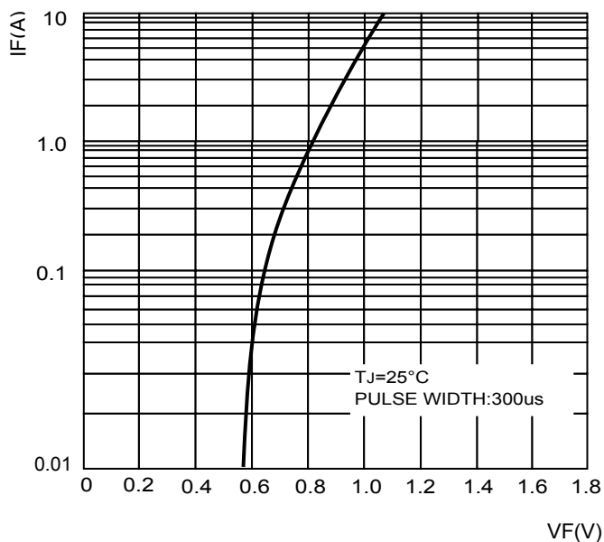
FIG.3-TYPICAL FORWARD CHARACTERISTICS
