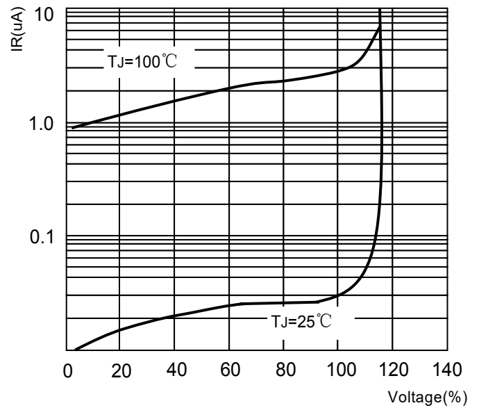
FIG.4-TYPICAL REVERSE CHARACTERISTICS
