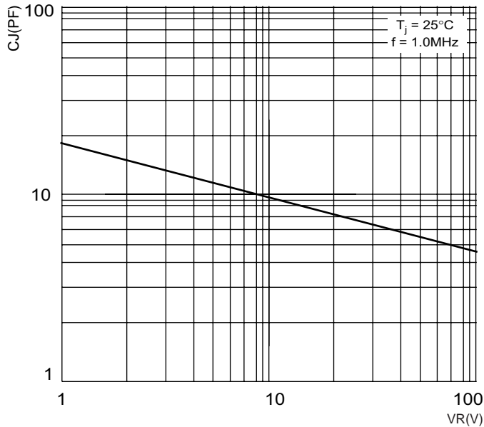
FIG5: Typical Junction Capacitance Per Diode
