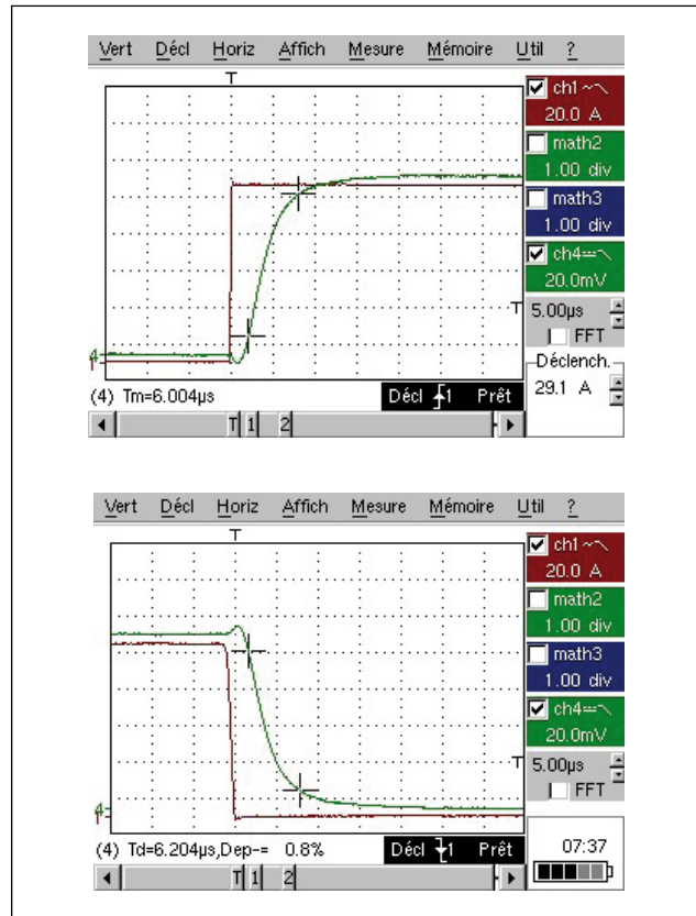
Pulse response
