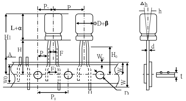
[ Fig. 2 (Diameter for \Phi 4 to \Phi 5 ) ]
