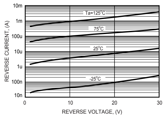
FIG. 2 - REVERSE CHARACTERISTICS
