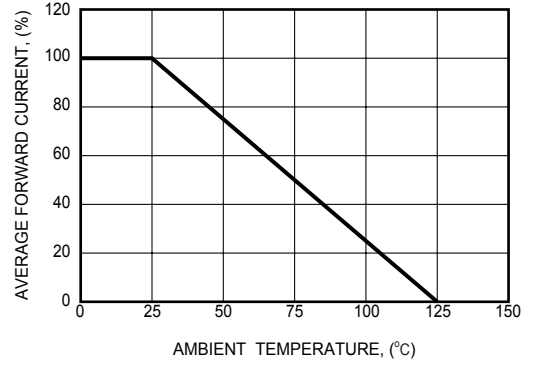
FIG. 4 - TYPICAL FORWARD CURRENT DERATING CURVE
