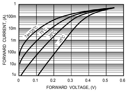
FIG. 1 - FORWARD CHARACTERISTICS
