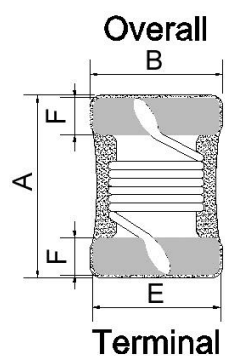
CS0201
