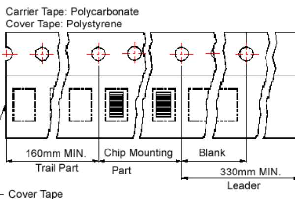
Tape Material
