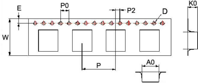
Tape Dimensions
