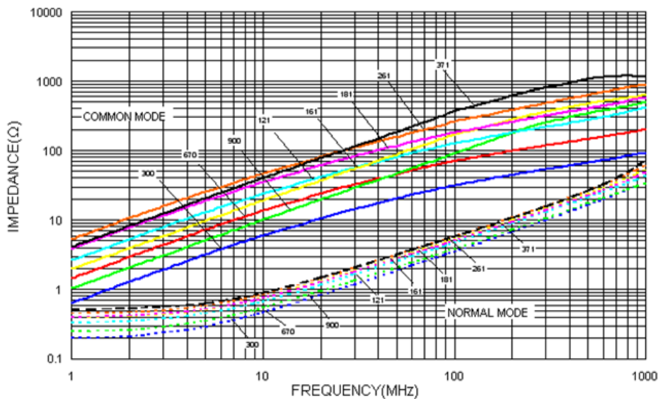
Typical Impedance vs. Frequency
