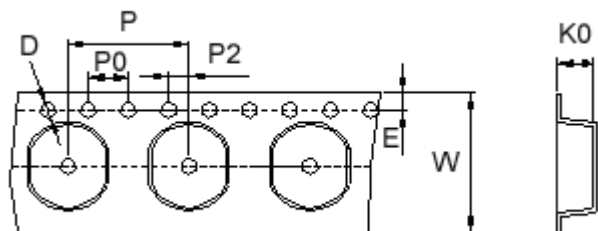
Tape Dimensions
