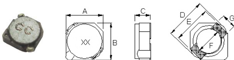
Dimension in mm
