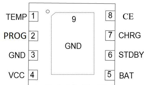
DFN2*2-8L
