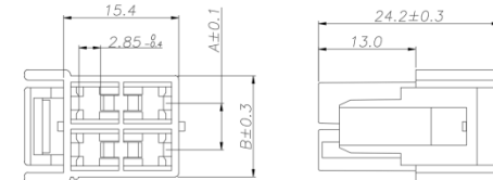
● Housing XD-C6200-2xNEY-05
