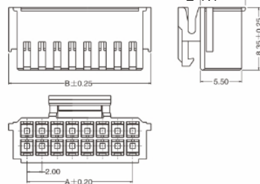
● Wafer
