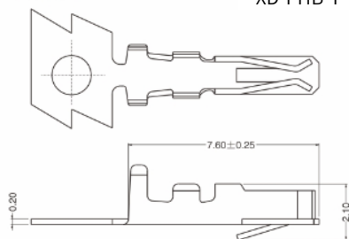
● Terminal XD-PHB-T
