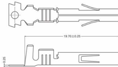
● Terminal XD-C6350-PT
