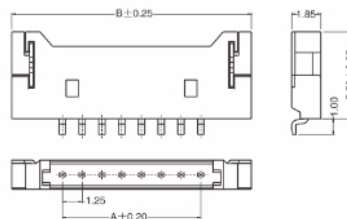
XD-CB1.25-NAWT
