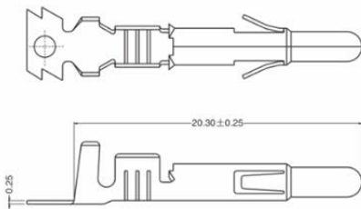
● Terminal XD-C6350-T
