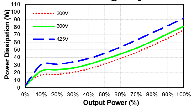
CFB750-300S24(N)-CMFD Pd Vs Po @25 Deg. C
