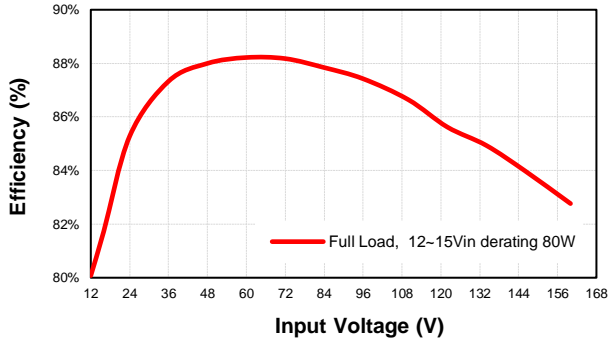
CQB100W14-72S05 Eff Vs Vin @25 Deg. C
