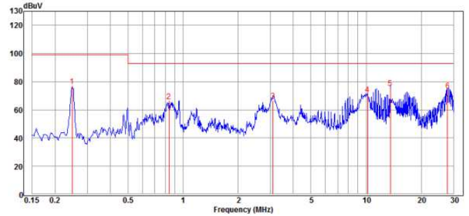
CQB50W12-72S24-CMFC
