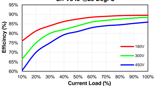
CQB75-300S12 Eff Vs Io @25 Deg. C
