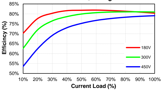
CQB75-300S3V3 Eff Vs Io @25 Deg. C
