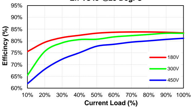
CQB75-300S05 Eff Vs Io @25 Deg. C
