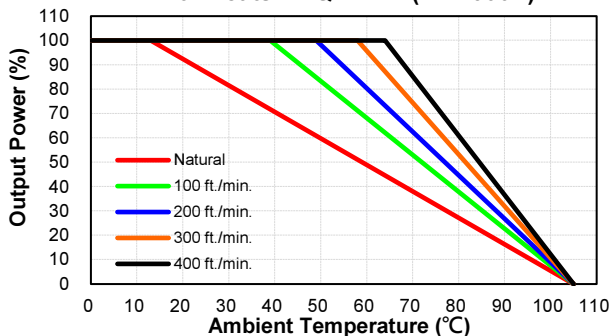
CQB75-300S05 Derating Curve with Heatsink QBL127 (Vin=300V)
