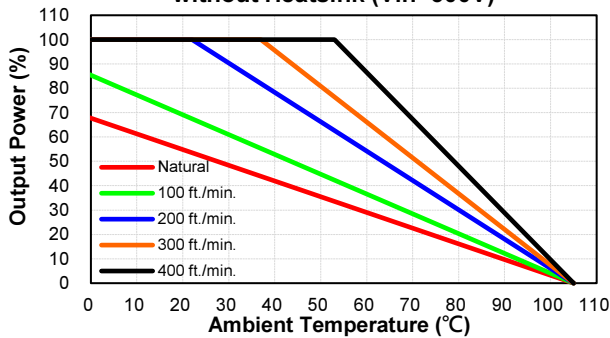
CQB75-300S05 Derating Curve without Heatsink (Vin=300V)
