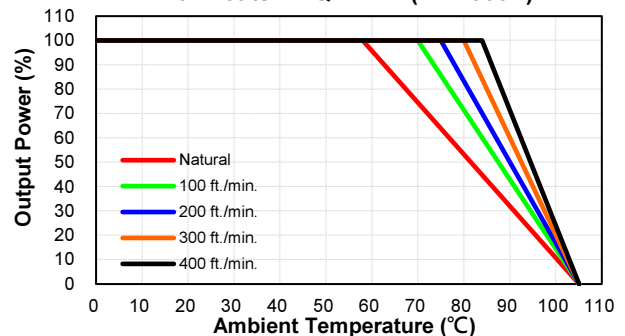
CQB75-300S12, 15, 24, 48 Derating Curve with Heatsink QBL127 (Vin=300V)
