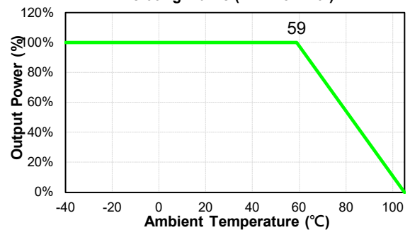
EC5SBW-XXS12,15, 48D12, 48D15-C(D)MF Derating Curve ( V_{in} =Nominal)
