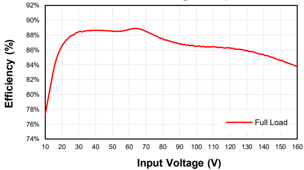
ECB40W18-72S15-ECRT Eff Vs Vin @25 Deg. C
