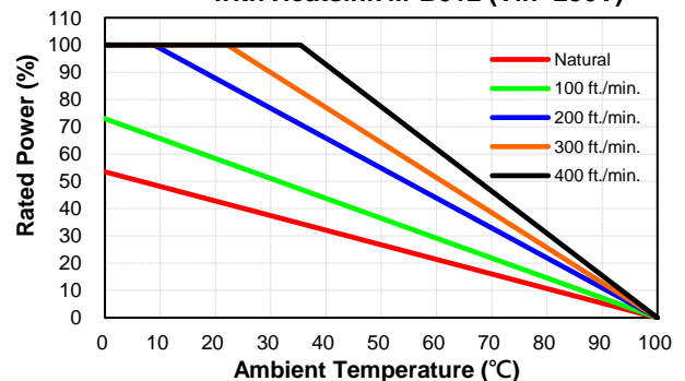
PDF700S240/280/480/560 Derating Curve with Heatsink M-B012 (Vin=230V)
