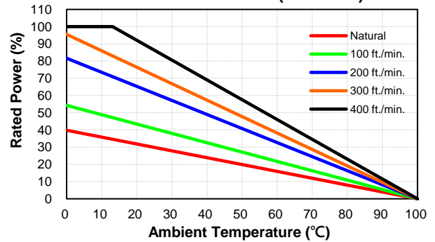
PDF700S120 Derating Curve with Heatsink M-B012 (Vin=230V)
