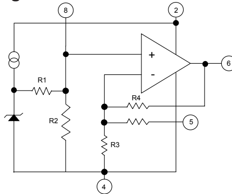
Figure 1. BLOCK DIAGRAM
