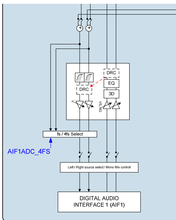
Figure 20 Ultrasonic (4FS) Signal Paths
