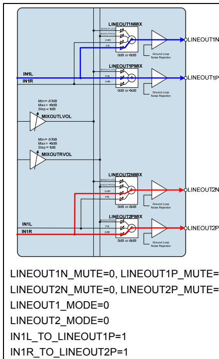
Figure 33 Differential Line Out from input PGA IN1L (to LINEOUT1) and IN1R (to LINEOUT2)
