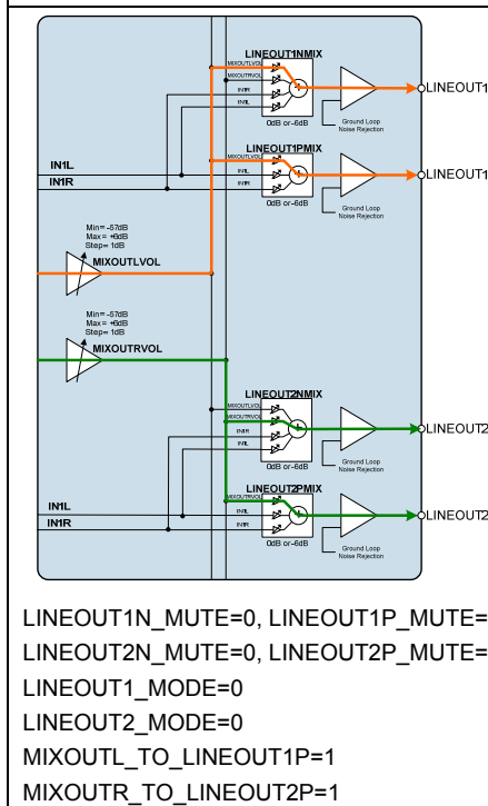
Figure 35 Stereo Differential Line Out from MIXOUTL and MIXOUTR
