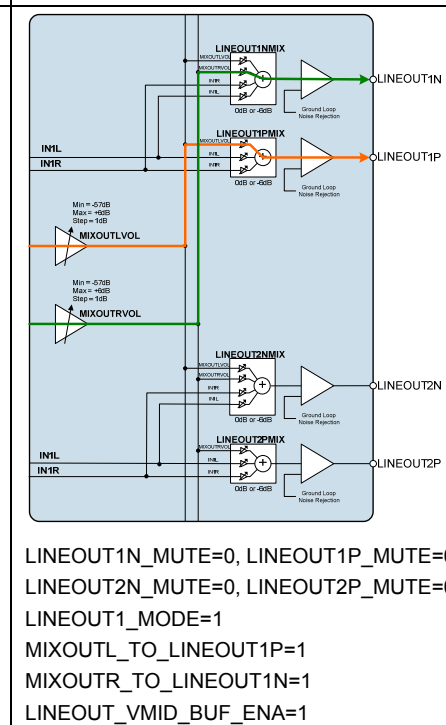
Figure 36 Stereo Single-Ended Line Out from MIXOUTL and MIXOUTR to LINEOUT1
