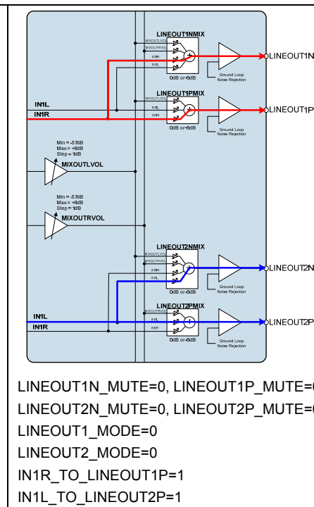
Figure 34 Differential Line Out from input PGA IN1R (to LINEOUT1) and IN1L (to LINEOUT2)
