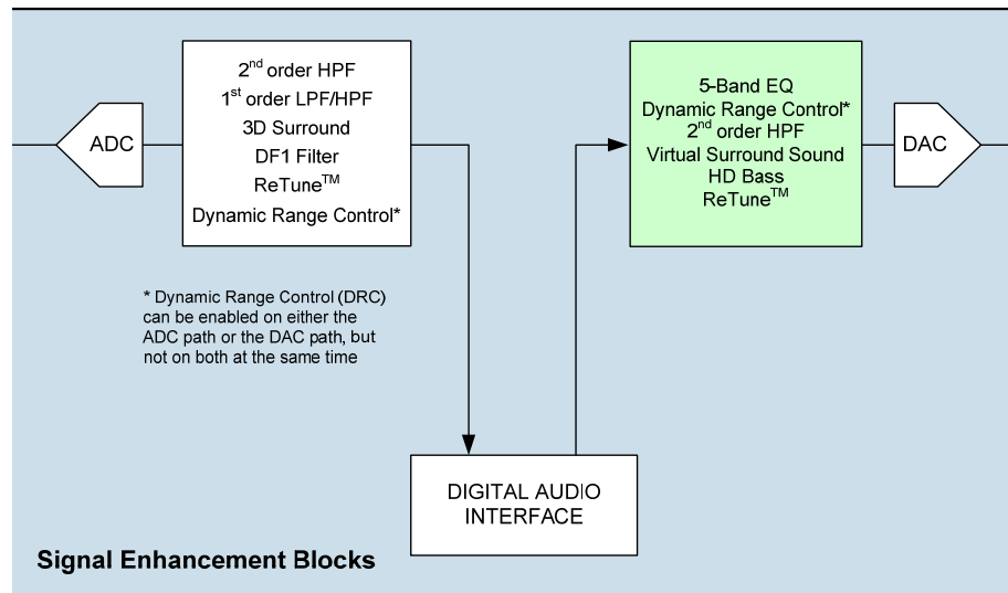
Figure 32 DAC Signal Enhancements
