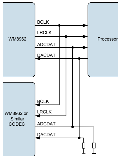
Figure 41 TDM with WM8962 as Master
