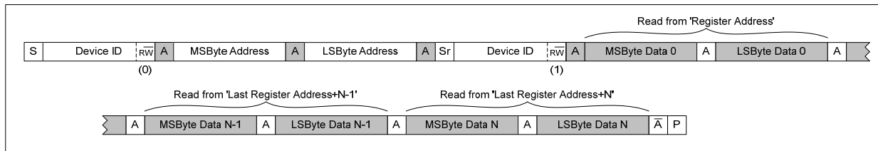
Figure 69 Multiple Register Read from Specified Address using Auto-increment
