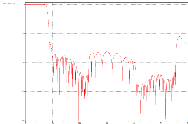
Figure 78 DAC Filter Response for 16k Sample Rate
