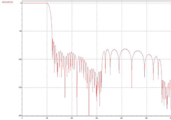
Figure 79 DAC Filter Response 22.05k Sample Rate
