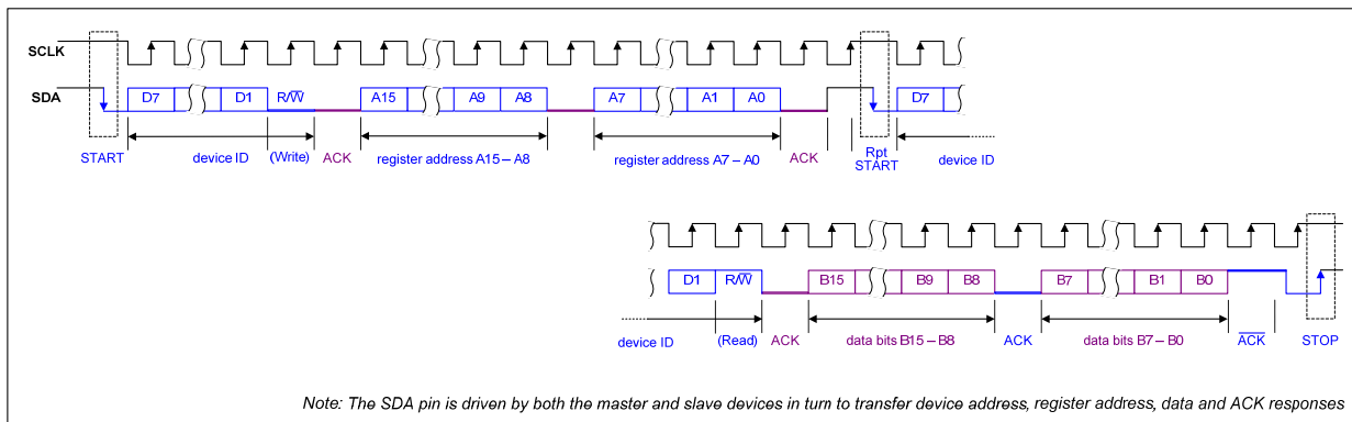
Figure 65 Control Interface 2-wire (I2C) Register Read
