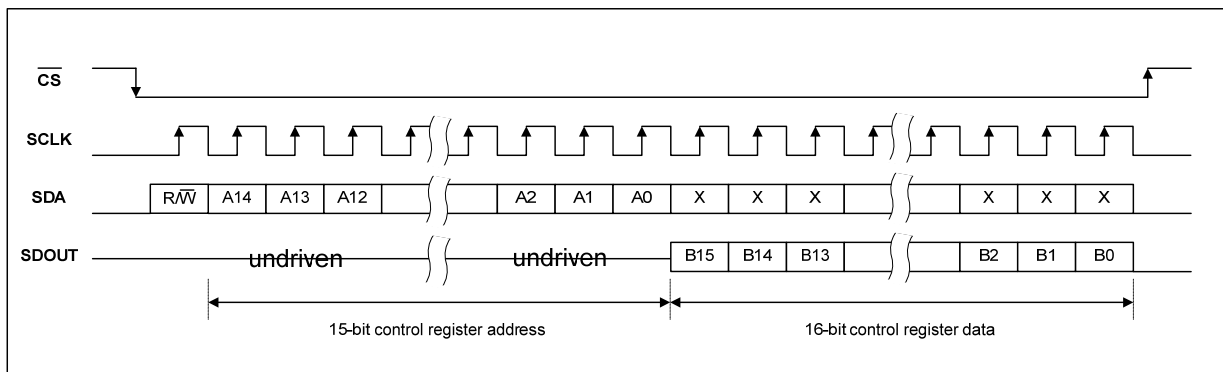
Figure 73 4-Wire Readback (Wired-'OR')
