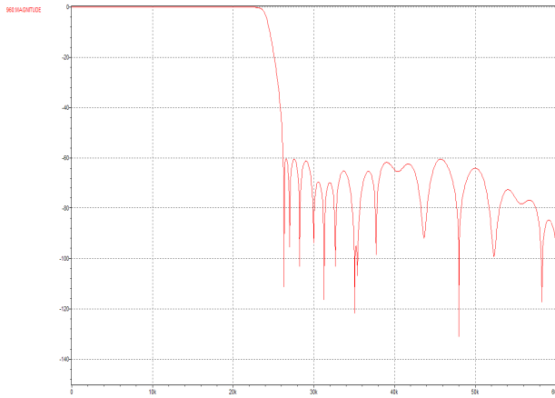
Figure 85 ADC Digital Filter Frequency Response (128OSR)
