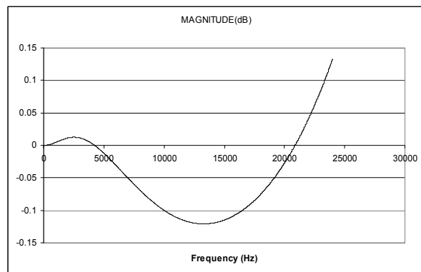
Figure 94 De-Emphasis Error (48kHz)
