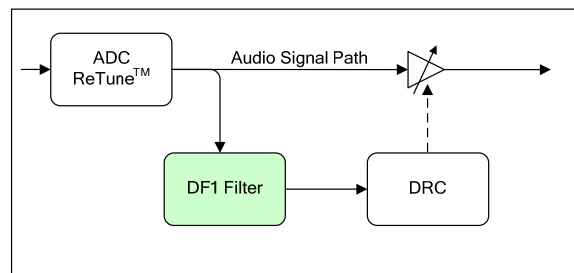
Figure 28 DF1 Filter on the DRC Signal Monitor Path
