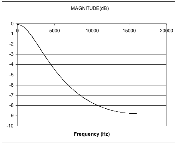
Figure 89 De-Emphasis Digital Filter Response (32kHz)
