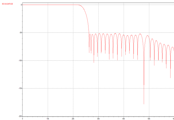
Figure 83 DAC Playback Filter Response for 48k Sample Rate
