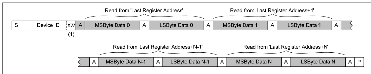
Figure 70 Multiple Register Read from Last Address using Auto-increment
