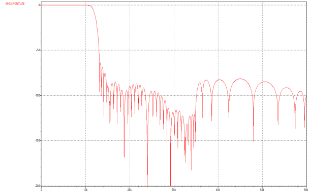
Figure 80 DAC Playback Filter Response for 24k Sample Rate
