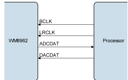
Figure 40 Slave Mode
