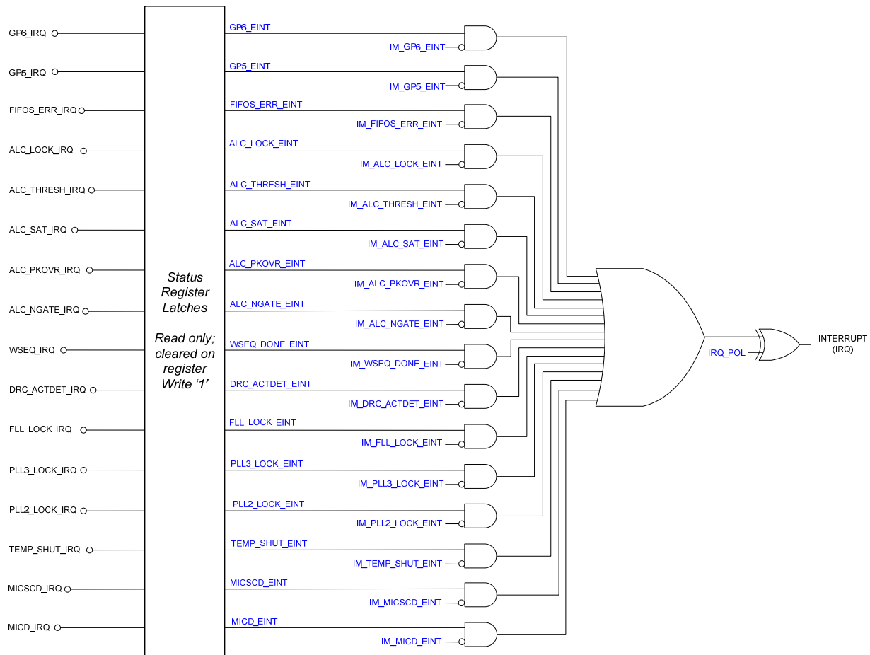
Figure 63 Interrupt Controller
