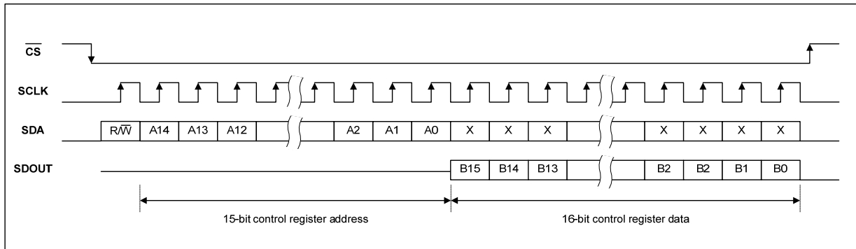
Figure 72 4-Wire Readback (CMOS)
