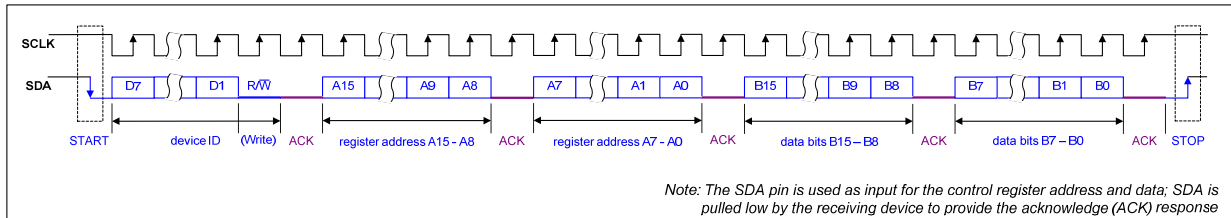
Figure 64 Control Interface 2-wire (I2C) Register Write
