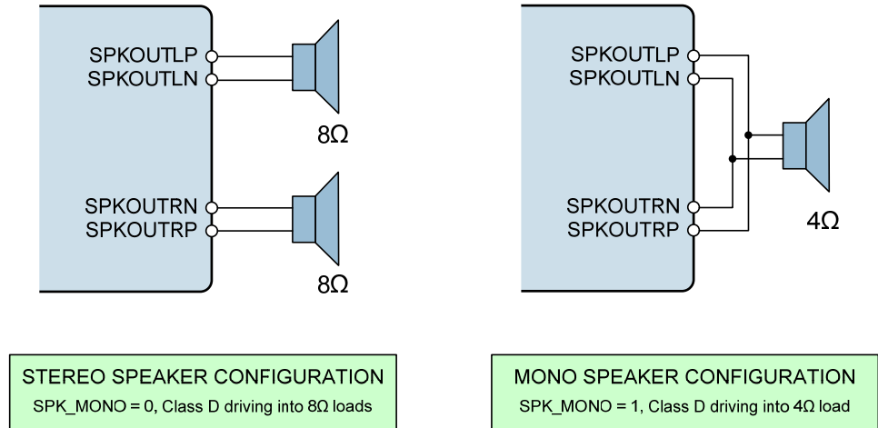
Figure 35 Mono and Stereo Speaker Output Configuration
