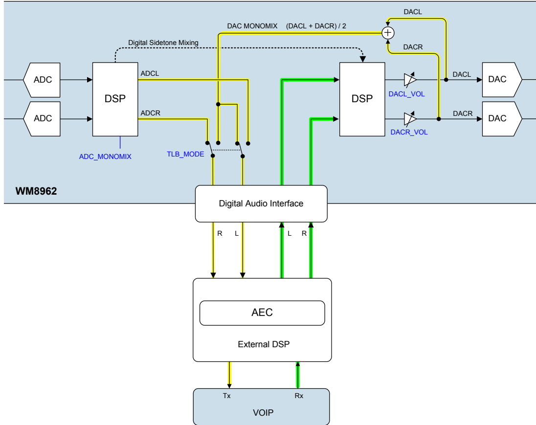
Figure 31 T-Loopback Signal Paths
