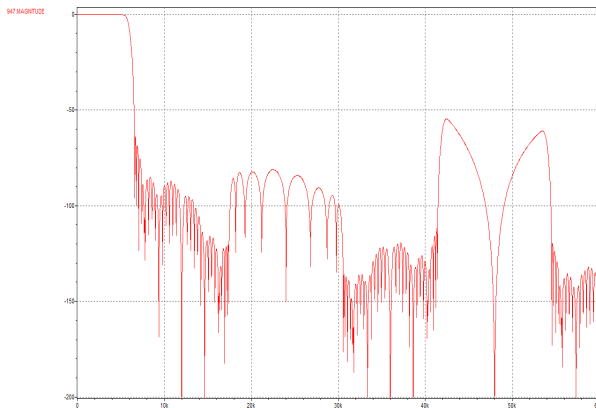
Figure 77 DAC Filter Response for 12k Sample Rate
