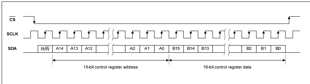
Figure 71 3-Wire Serial Control Interface
