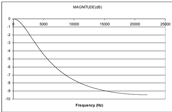
Figure 91 De-Emphasis Digital Filter Response (44.1kHz)
