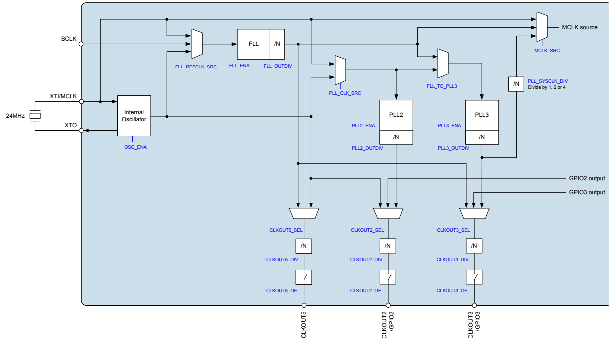
Figure 59 Clock Generation Block Diagram
