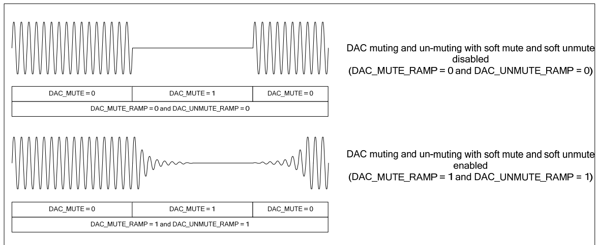
Figure 33 DAC Mute Control
