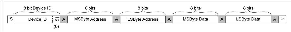
Figure 66 Single Register Write to Specified Address
