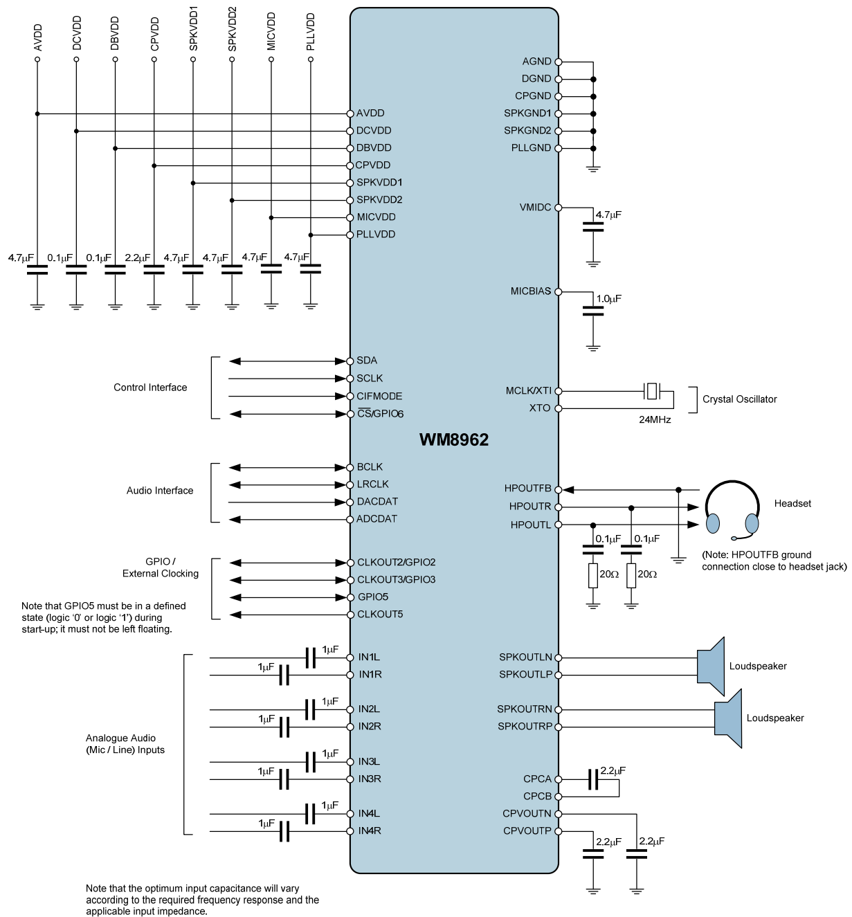
Figure 98 WM8962 Recommended External Components
