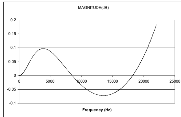
Figure 92 De-Emphasis Error (44.1kHz)
