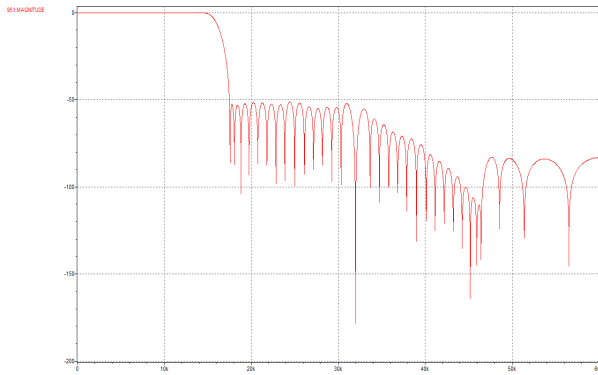
Figure 81 DAC Playback Filter Response for 32k Sample Rate
