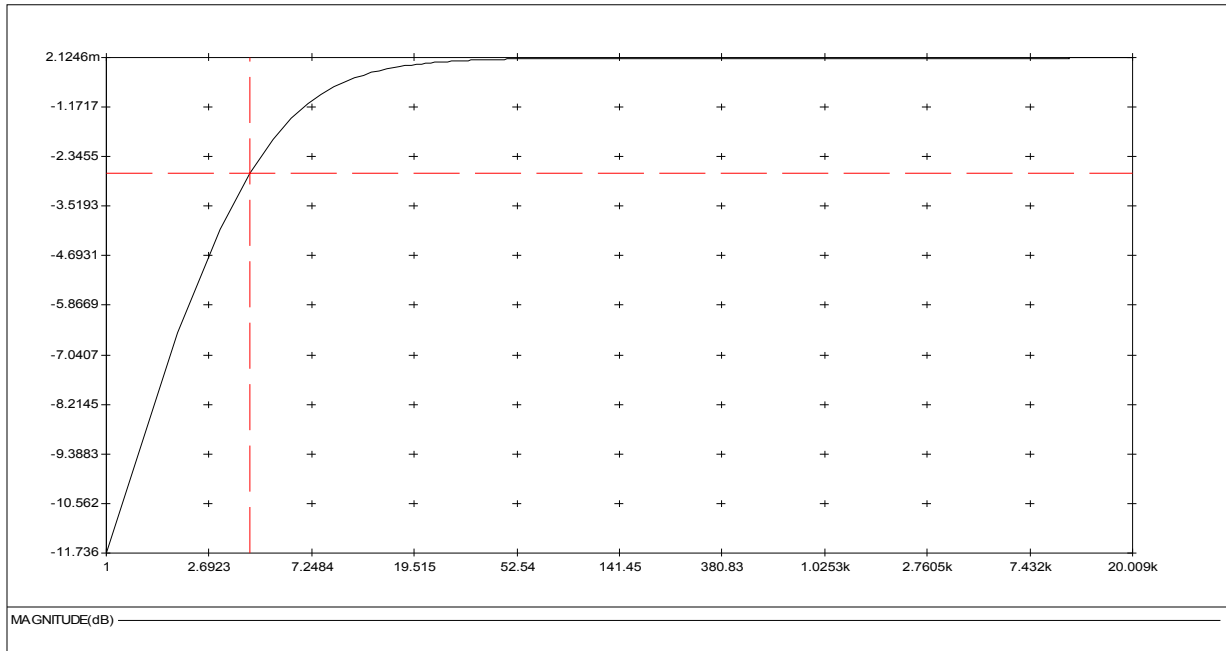
Figure 87 ADC Digital High Pass Filter Frequency Response (48kHz, Hi-Fi Mode, ADC_HPF_CUT[1:0]=00)
