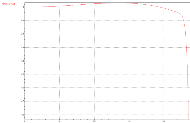
Figure 86 ADC Digital Filter Passband Ripple (128OSR)
