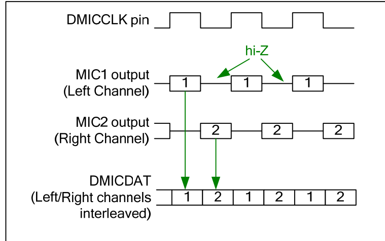
Figure 22 Digital Microphone Interface Timing
