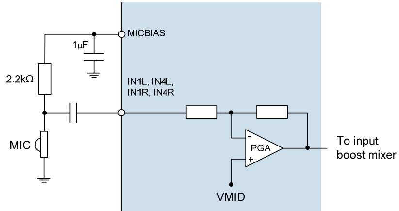
Figure 96 Single Ended Microphone Connection
