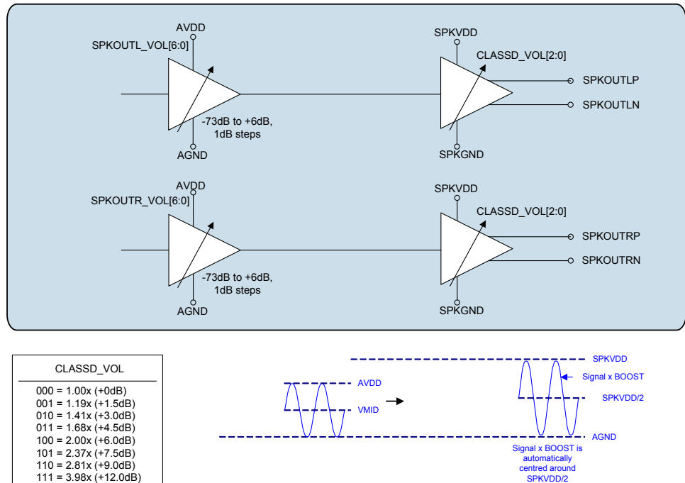
Figure 36 Speaker Output Configuration and AC Boost Operation
