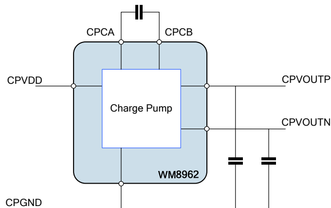
Figure 38 Charge Pump External Connections
