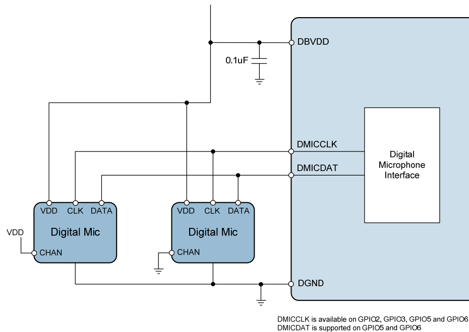
Figure 21 Digital Microphone Input
