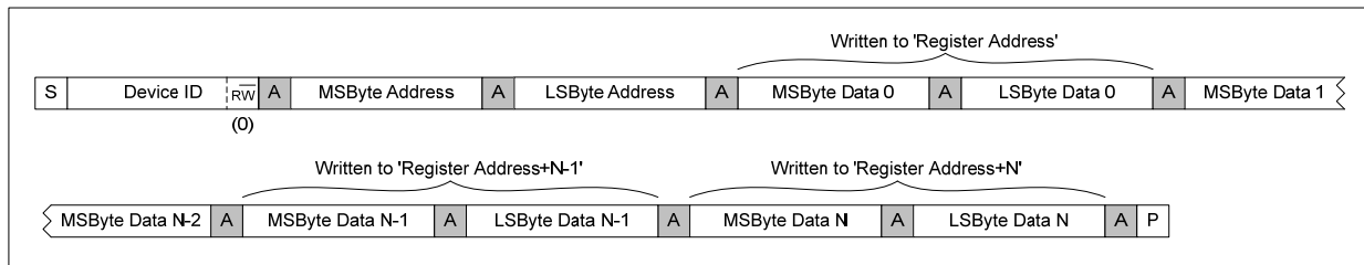
Figure 68 Multiple Register Write to Specified Address using Auto-increment
