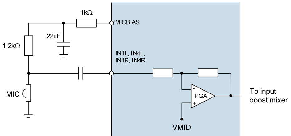
Figure 97 Microphone Connection, with MICBIAS filter components
