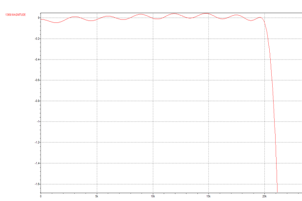
Figure 84 DAC Playback Filter Passband Ripple for 44.1k Sample Rate (MCLK=11.2896MHZ)
