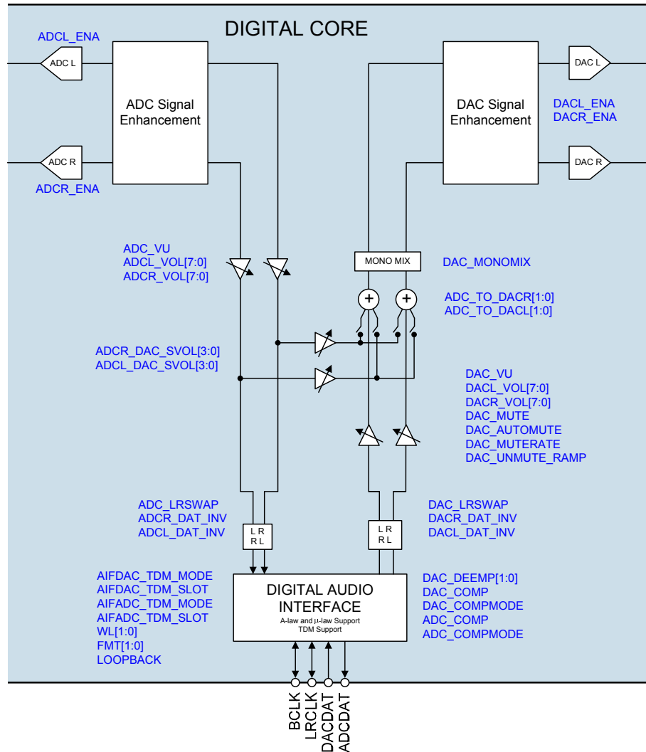
Figure 30 Digital Mixing Paths
