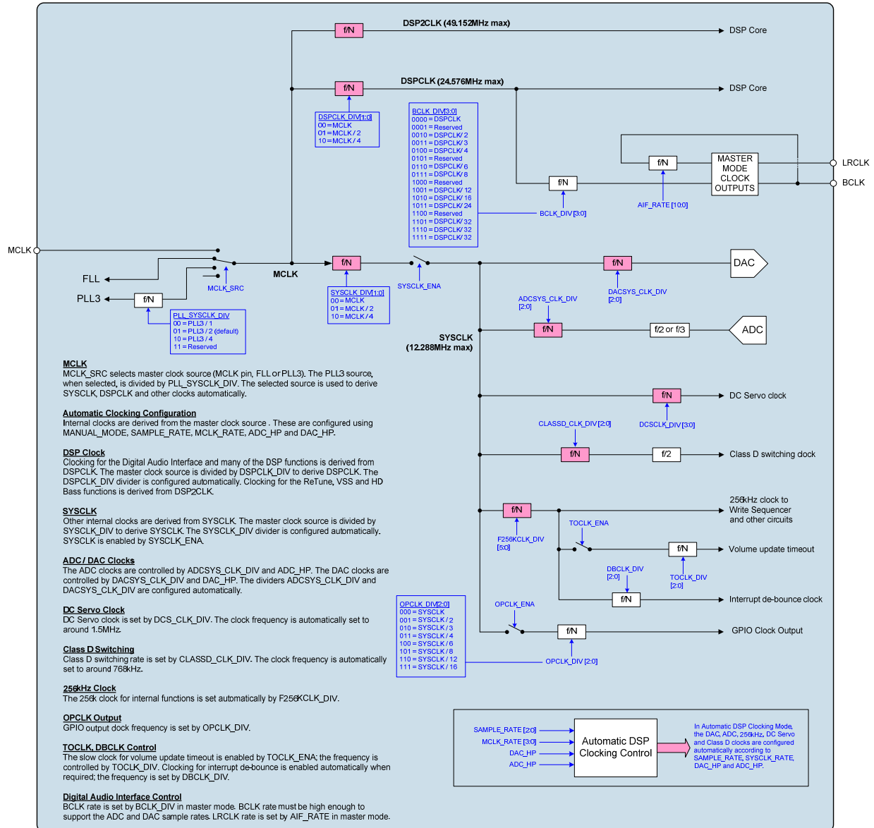
Figure 58 SYSCLK and Internal Clocking Scheme
