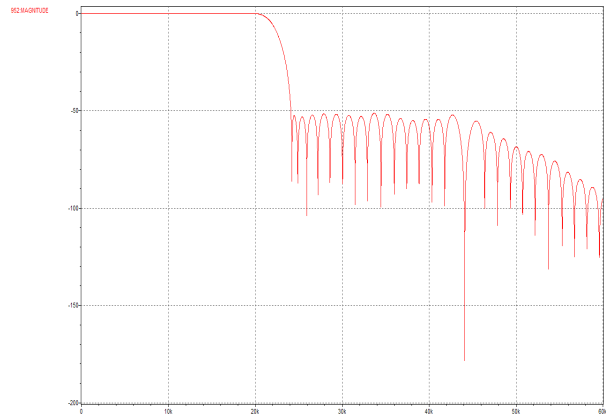
Figure 82 DAC Playback Filter Response for 44.1k Sample Rate
