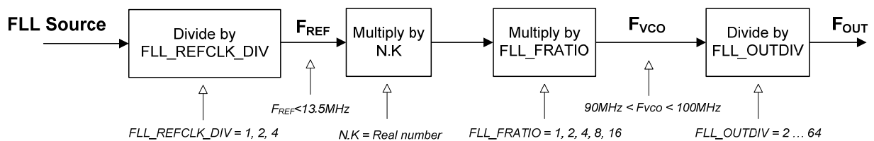
Figure 61 FLL Configuration
