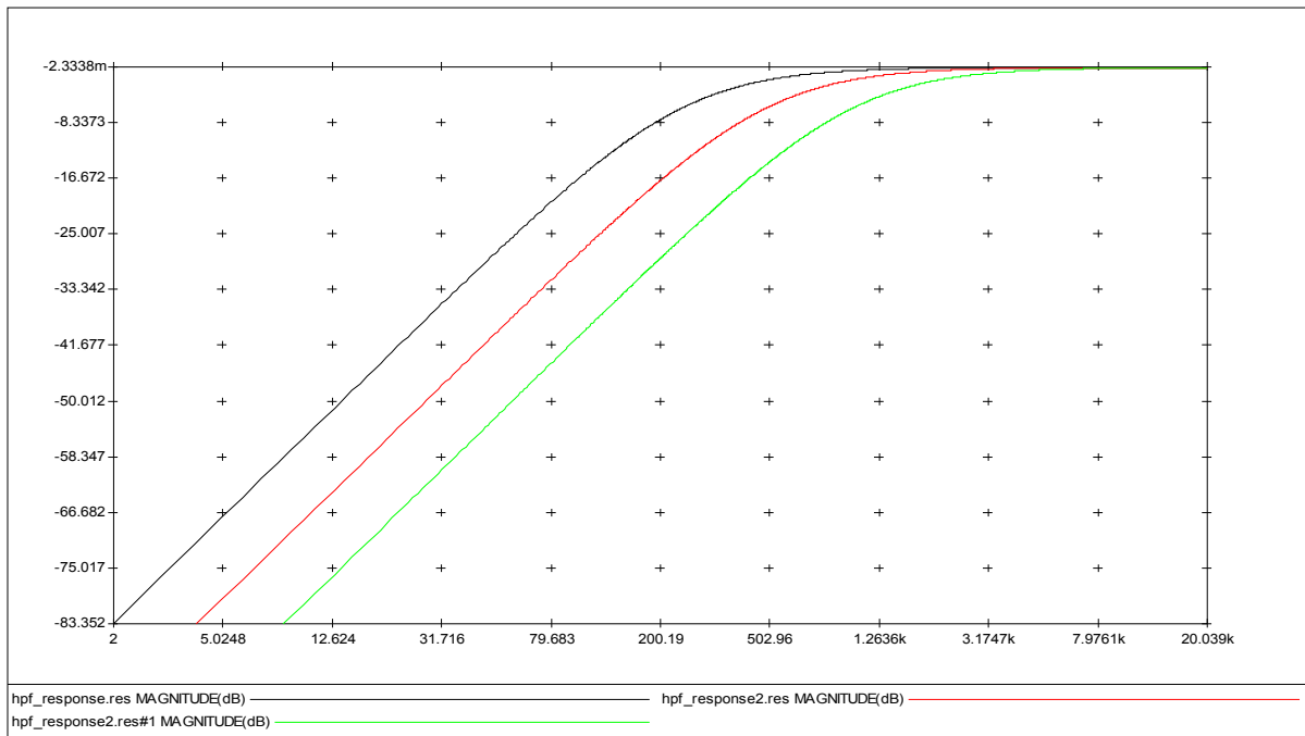
Figure 88 ADC Digital High Pass Filter Ripple (48kHz, Voice Mode, ADC_HPF_CUT=01, 10 and 11)
