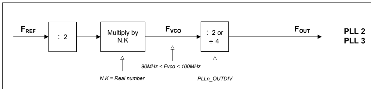
Figure 62 PLL Frequency Control
