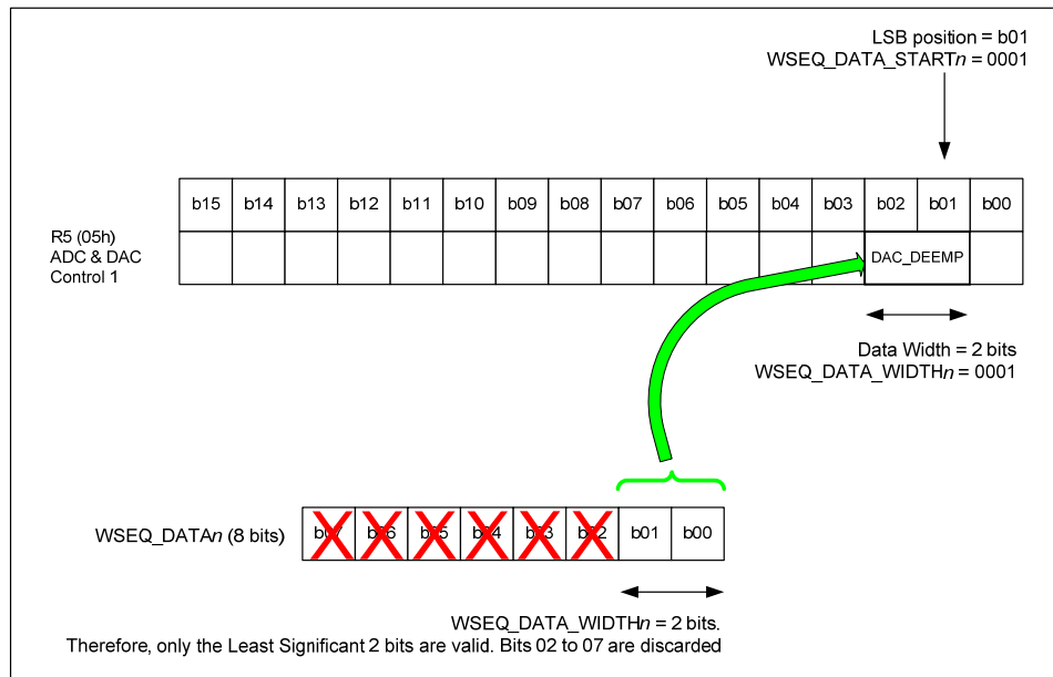
Figure 74 Control Write Sequencer Example
