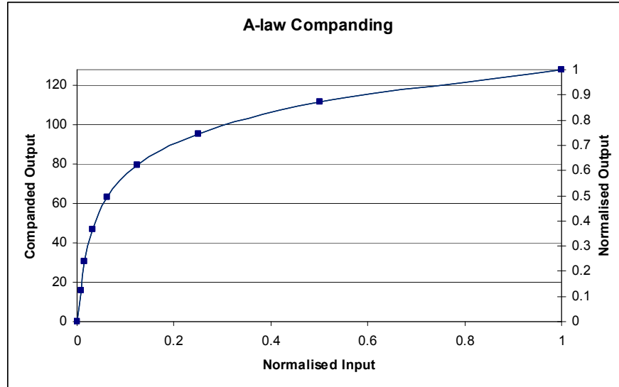
Figure 57 A-Law Companding
