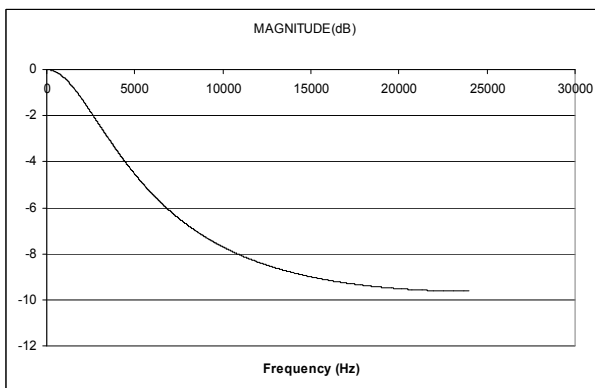
Figure 93 De-Emphasis Digital Filter Response (48kHz)
