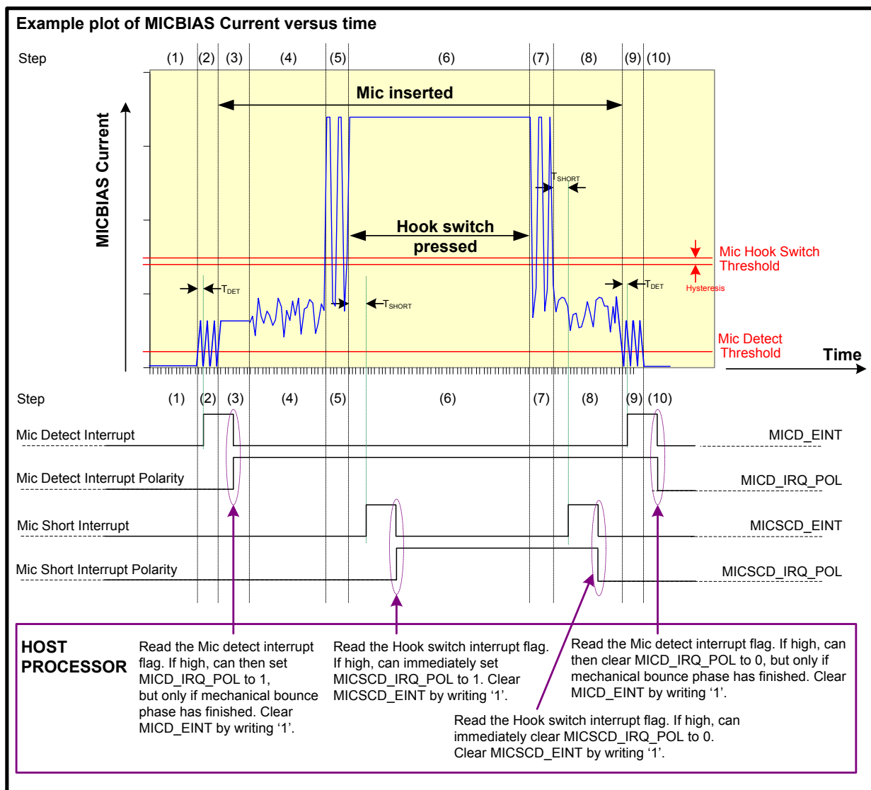
Figure 99 Mic Insert and Hook Switch Detect: Example MICBIAS Current Plot
