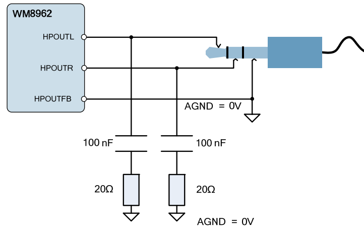
Figure 37 Zobel Network Components for HPOUTL and HPOUTR
