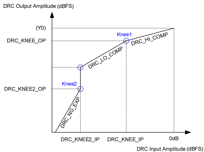
Figure 29 DRC Response Characteristic
