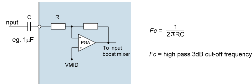
Figure 95 Audio Input Path DC Blocking Capacitor
