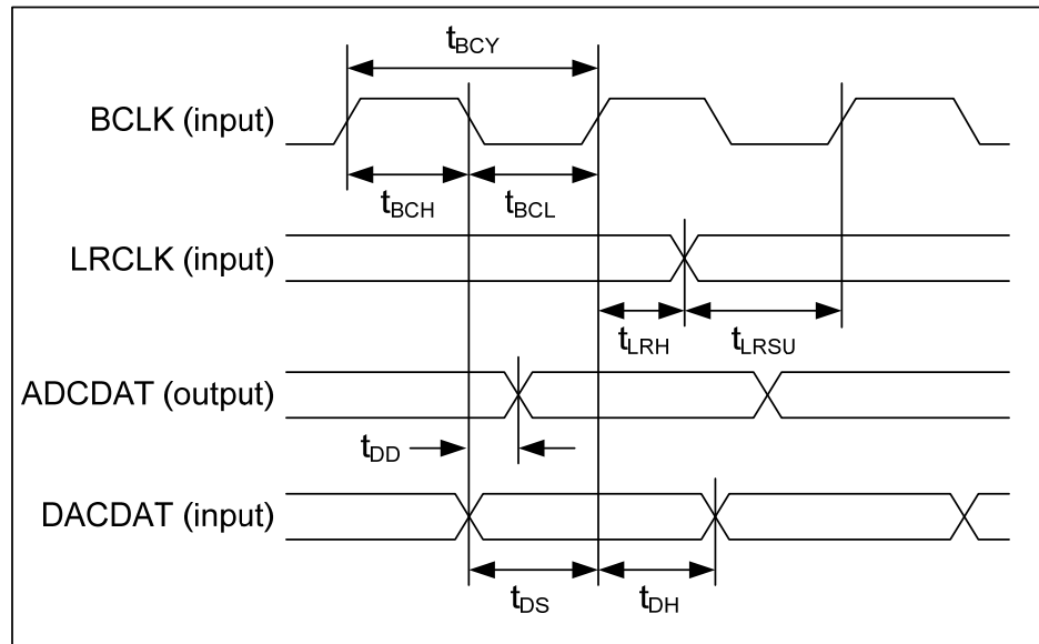
Figure 4 Audio Interface Timing – Slave Mode
