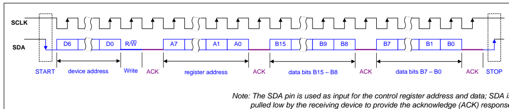
Figure 8 Control Interface I 2 C Register Write
