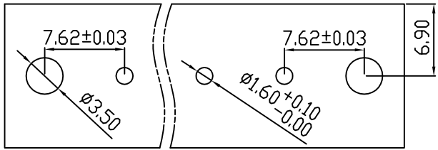
PCB LAYOUT
