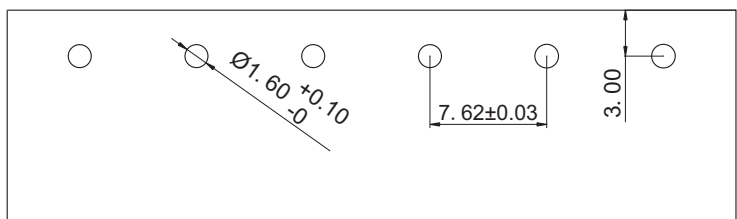
PCB Layout
