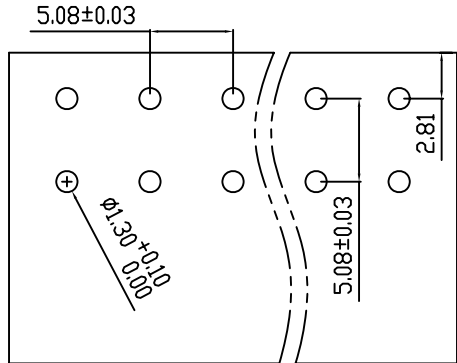
PCB LAYOUT
