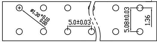
PCB LAYOUT
